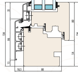
SYSTEM NATURO 80 ALU GEMINI CLASSIC Innere Fensterbankfräsung
