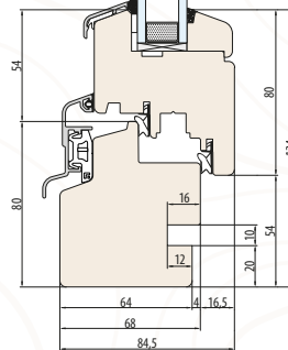
SYSTEM NATURO 68 Innere Fensterbankfräsung
