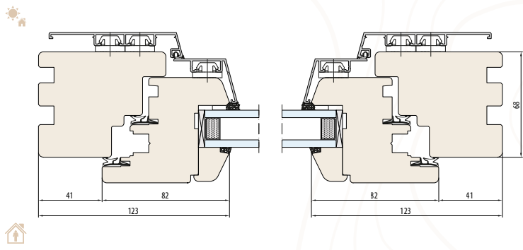
SYSTEM NATURO 68 ALU RENO LINE
