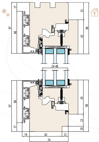
SYSTEM ESPERIA LIFE 74 ALU Innere Fensterbankfräsung
